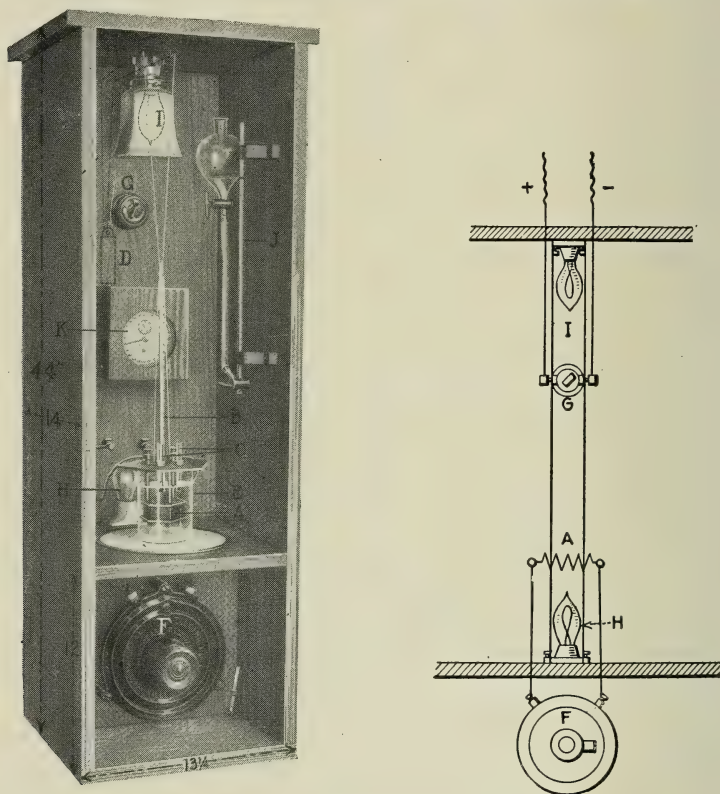
FIG. 175.—K. & S. Fusing-Point Tester.
